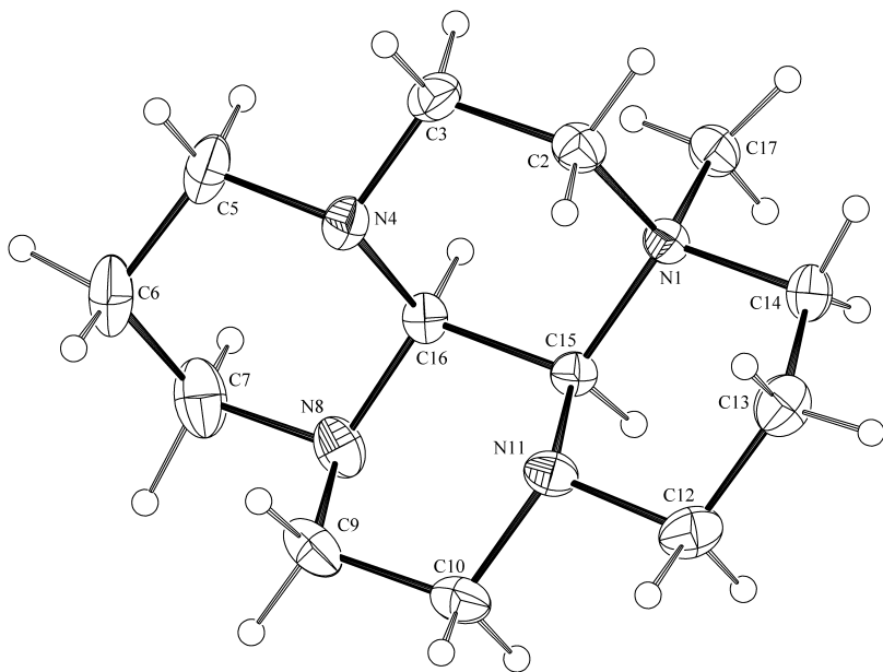
FIG. 1 ORTEP representation of molecular structure of (Me-2) + in crystal structure of 5b
