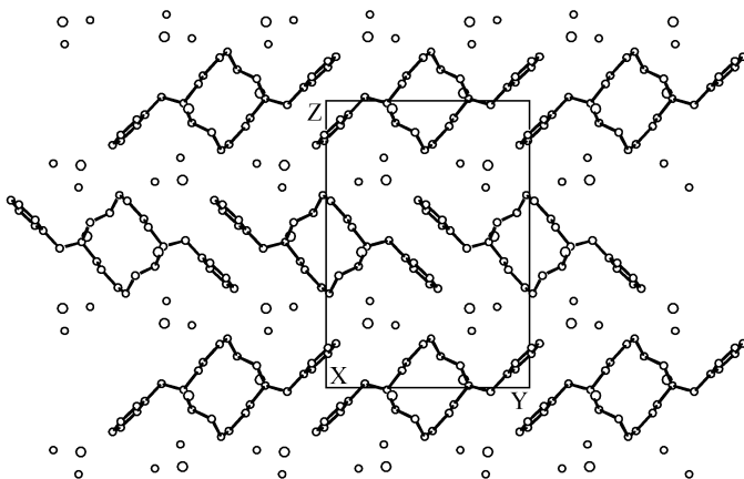
FIG. 6 Crystal packing in structure of 4a ·4HCl·4H 2 O
